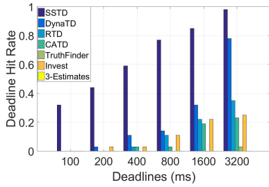
(a) Boston Bombing Trace
