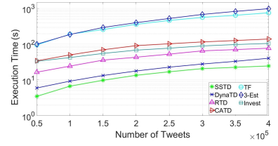
(c) College Football Trace
