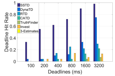
(c) College Football Trace
