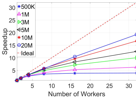
Fig. 7. Scalability of SSTD Scheme
