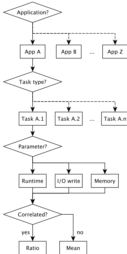
Figure 5: Estimation process for one parameter.
