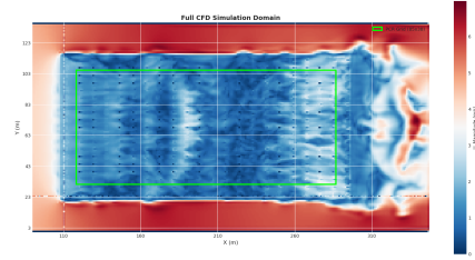
Fig. 2: CFD-simulated wind speed (m/s) at Z = 1 m within the CUPS structure. Colors indicate wind speed, with predominant airflow from left to right. The green rectangle outlines the growing region.
