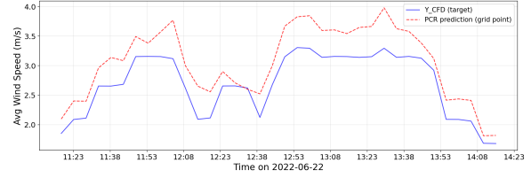
Fig. 5: Comparison of CFD ground truth (solid) and PC-R predictions (dashed) at a representative interior grid point ( x=40.3 m, y=48.1 m, z=5.0 m, relative to the growing-region origin) over the full Period 2 duration in Figure 4. The model is trained exclusively on Period 1; at this point, prediction accuracy is MAE=0.37 m/s, R^2=0.39 , RMSE=0.40 m/s.
