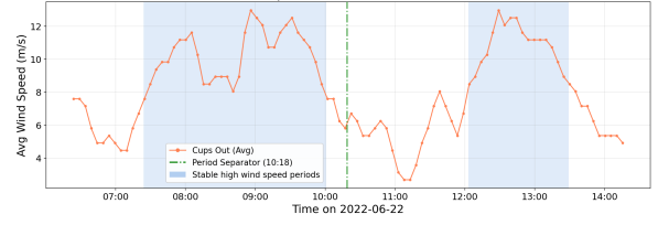
Fig. 4: Historical wind measurements outside the CUPS spanning Period 1 and Period 2, separated at 10:18 (green line). Each period contains an extended stable high-wind regime (shaded), reaching comparable peak magnitudes ( \approx 13 m/s), bounded by lower, more variable conditions.
