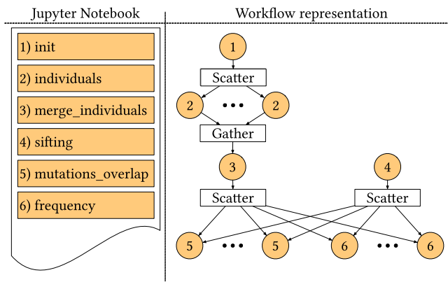
Fig. 9. Graphical representation of the Jw execution plan for the 1000-genome workflow.
