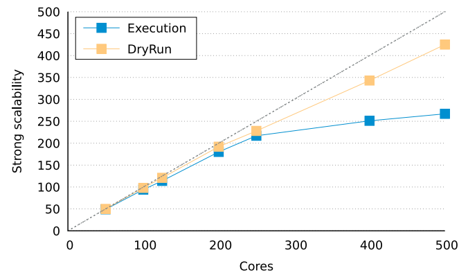
Fig. 10. Speedup obtained executing the 1000-genome workflow on the HPC4AI Cloud. The blue curve refers to a real execution. The orange curve shows a DryRun of the same workflow aimed at assessing Jw overhead (the business code is substituted with sleeps matching execution time).
