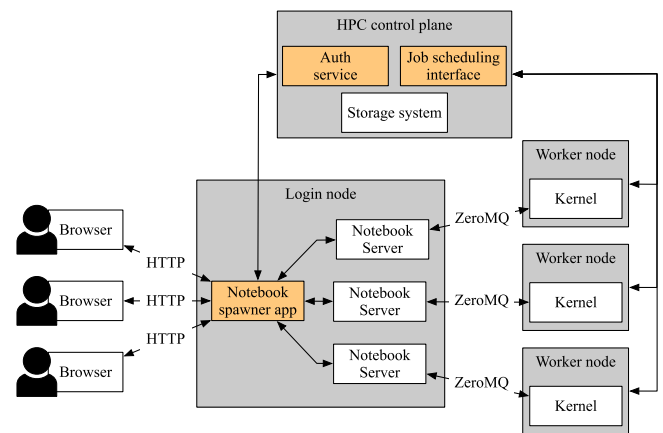
Fig. 1. Sketch of the common architecture of a HPC Jupyter interface. Orange blocks usually need to be developed or extended to integrate Jupyter in the existing software stack.
