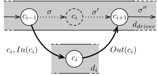
Fig. 3. Interactive remote execution of a configuration \langle [c_i, d_i], \sigma \rangle . When d_i \neq d_{driver} , both code c_i and true data dependencies In(c_i) must be transferred to d_i . After that, the return values Out(c_i) can be transferred back to d_{driver} .
