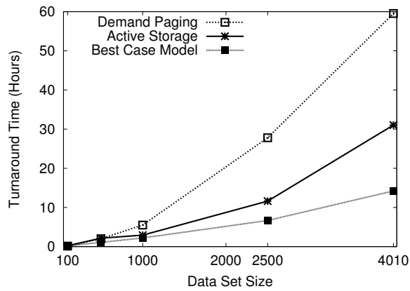
Figure 6. Performance of a Biometric All-Pairs Workload The biometric face comparison function takes 1s to compare two 1.25MB images.
