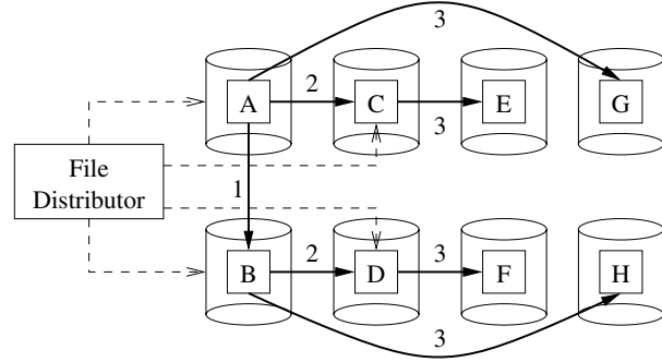
Figure 3. File Distribution via Spanning Tree
