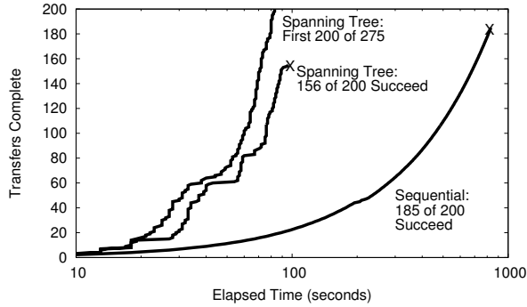
Figure 3. File Distribution via Spanning Tree
