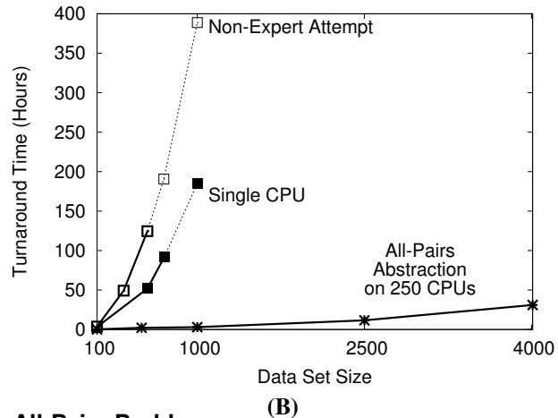
Figure 1. The All-Pairs Problem
