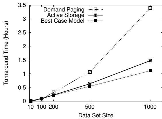
Figure 7. Performance of a Data Mining All-Pairs Workload The data mining function takes .25 seconds to compare two 700KB items.
