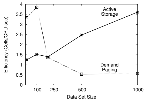
Figure 7. Performance of a Data Mining All-Pairs Workload The data mining function takes .25 seconds to compare two 700KB items.
