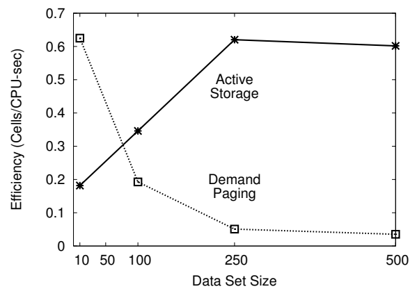
Figure 8. Performance of a Synthetic All-Pairs Workload This function takes 1s for two 12MB data items, 10 times the data rate of the biometric workload.
