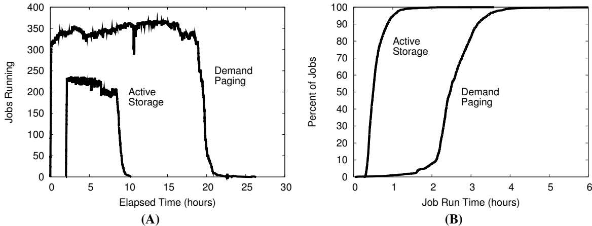
Figure 5. Time Variance in a Shared Computing System
